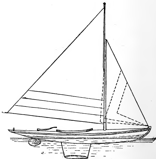
SAIL PLAN OF FIN-KEEL.
